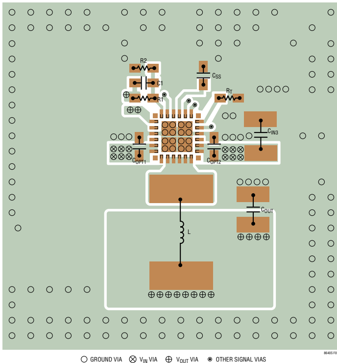
(a) LT8640S
