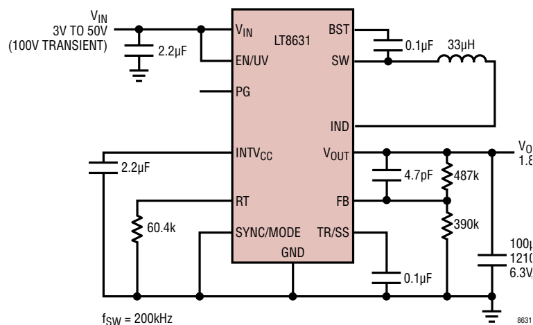
200kHz, 1.8V, 1A Step-Down Converter
