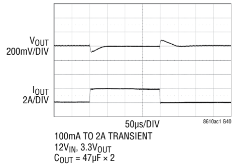
LT8610AC-1 Transient Response
