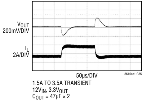
LT8610AC Transient Response
