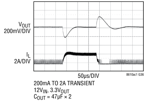
LT8610AC Transient Response
