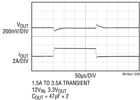
LT8610AC-1 Transient Response
