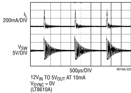
Switching Waveforms
