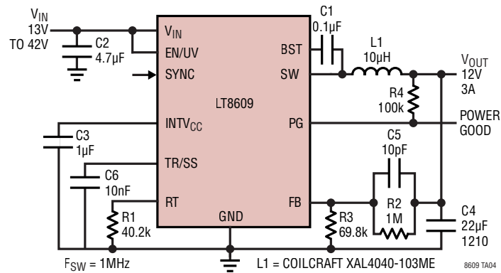
12V Step-Down
