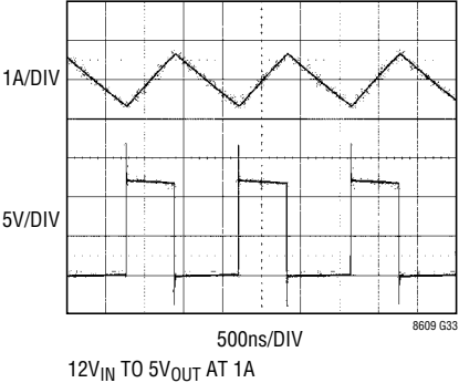
Switching Waveforms
