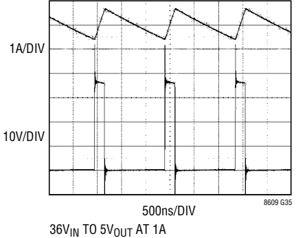
Switching Waveforms
