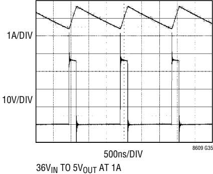
Switching Waveforms
