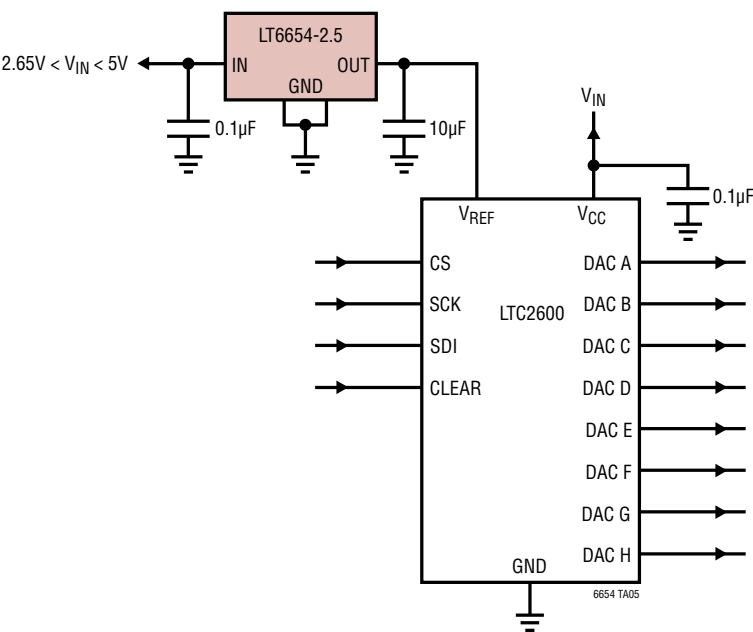
Octal DAC Reference
