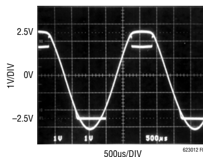
Figure 2. V_S = \pm 2.5\text{V} , A_V = 1 with Large Overdrive
