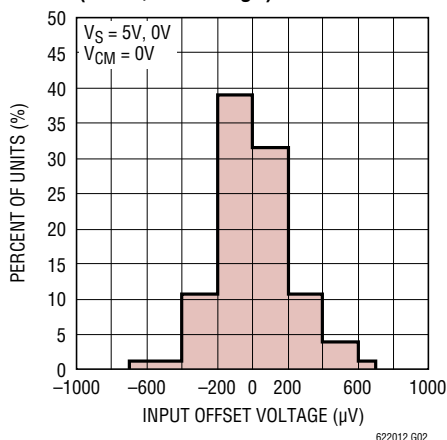
V_{OS} Distribution, V_{CM} = 0V (SOT5, PNP Stage)
