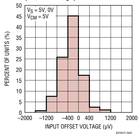
V_{OS} Distribution, V_{CM} = 5V (S8, NPN Stage)
