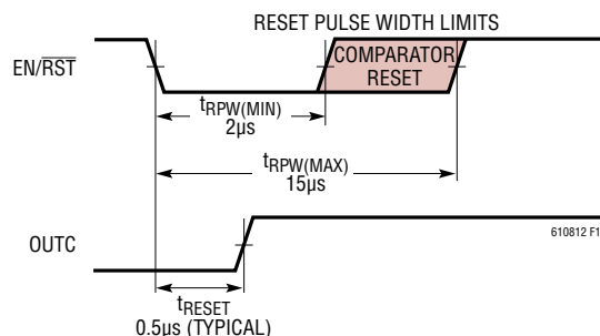
Figure 16. Comparator Reset Functionality
