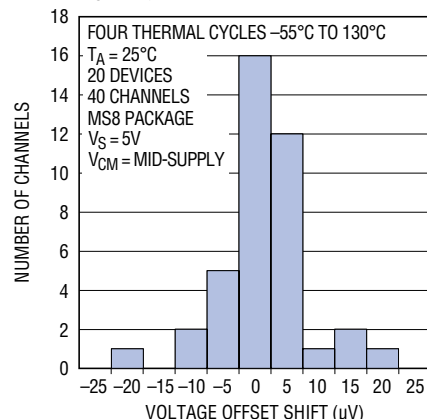
Voltage Offset Shift vs Thermal Cycling
