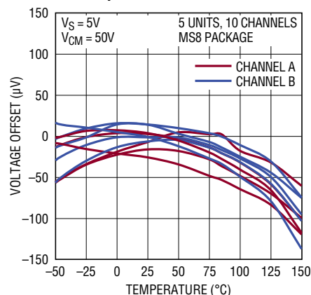
Over-The-Top Voltage Offset vs Temperature
