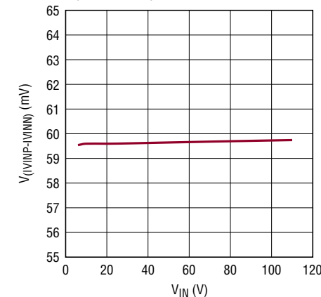
V (IVINP-IVINN) Threshold vs V IN
