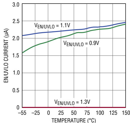
EN/UVLO Current vs Temperature
