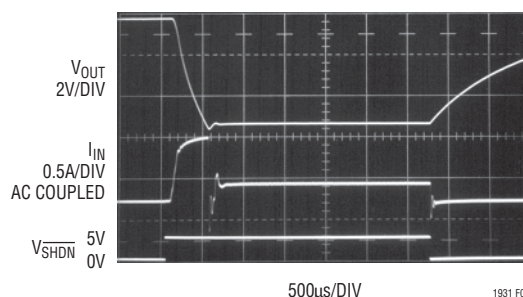
Figure 6. Start-Up Waveforms for 5V to -5V Application (Figure 1). No Soft-Start Circuit. V_{OUT} Reaches -5V in 500μs; Input Current Peaks at 800mA
