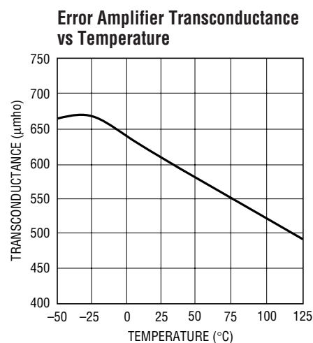
LT1776 G12
