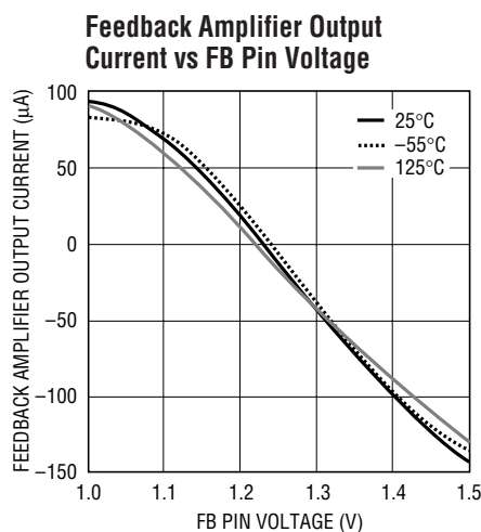
LT1776 G11
