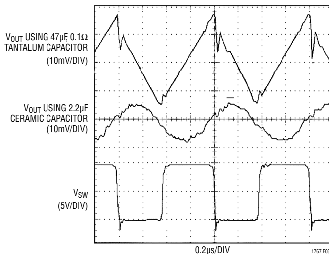
Figure 3. Output Ripple Voltage Waveform
