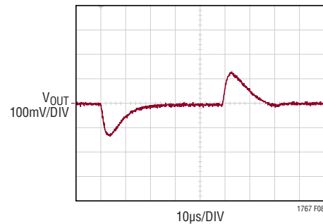
Figure 8. Oscilloscope Shows the Output Voltage Response to a Load Current Transient from 0.3A to 1A. The Compensation Network Results in Fast, Damped Response. (Front Page Schematic, 12V in to 3.3V out)
