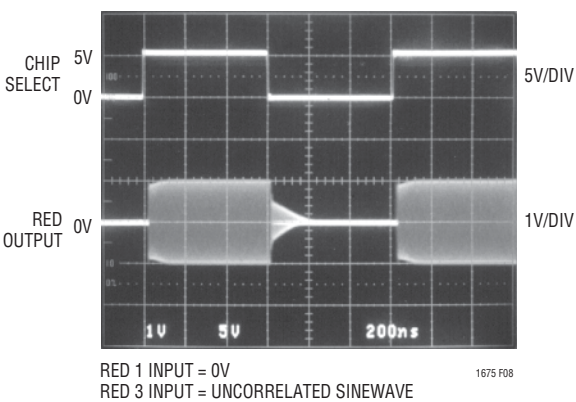
Figure 8. 4-Input Router Toggling
