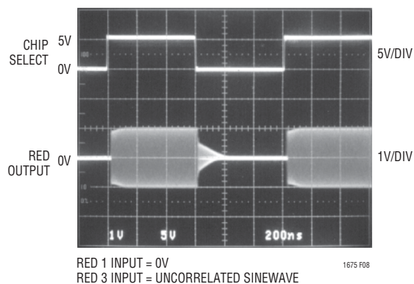
Figure 8. 4-Input Router Toggling
