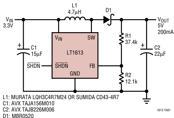
Figure 1. 3.3V to 5V 200mA DC/DC Converter
