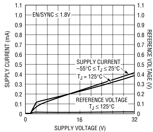
Shutdown Mode Supply Current and Reference Voltage
