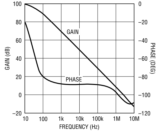
Current Amplifier Open-Loop Gain and Phase
