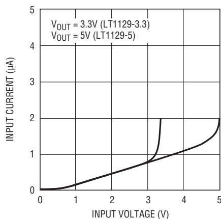
Figure 4. Input Current
