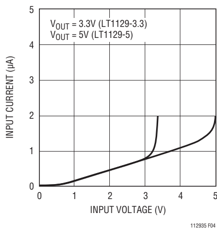
Figure 4. Input Current
