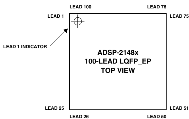
Figure 49. 100-Lead LQFP_EP Lead Configuration (Top View)
