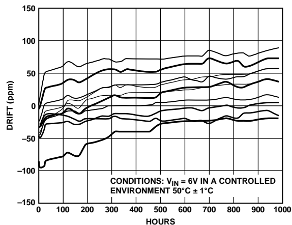
Figure 25. ADR381 Long-Term Drift
