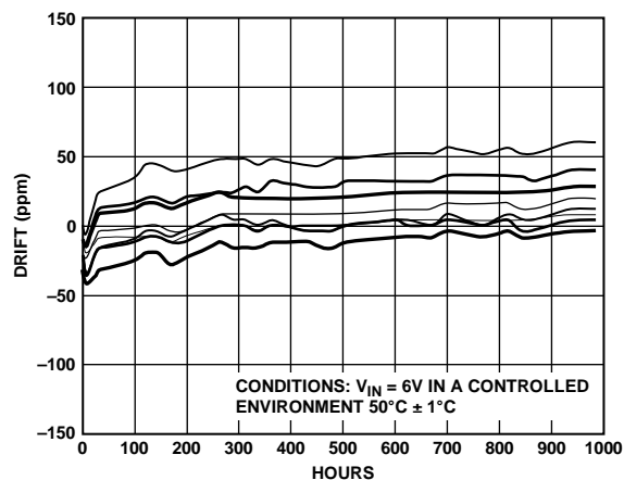
Figure 24. ADR380 Long-Term Drift
