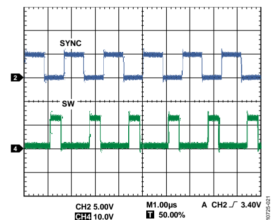
Figure 21. External Synchronization
