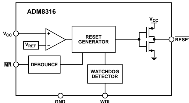
Figure 1. ADM8316
