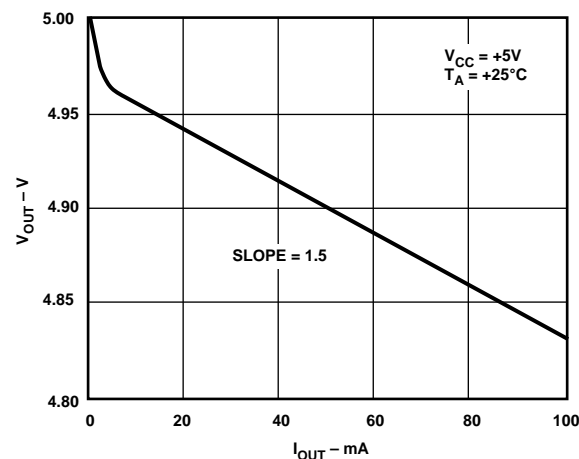
Figure 8. V_{OUT} vs. I_{OUT} Normal Operation
