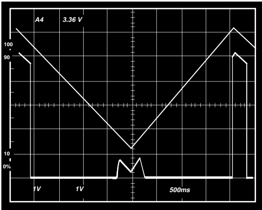
Figure 12. RESET Output Voltage vs. Supply Voltage
