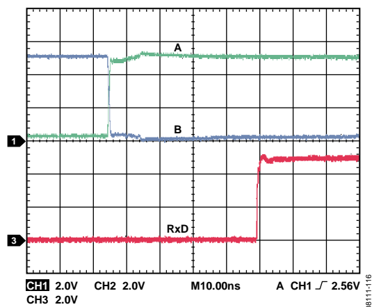
Figure 16. ADM2582E Receiver Propagation Delay
