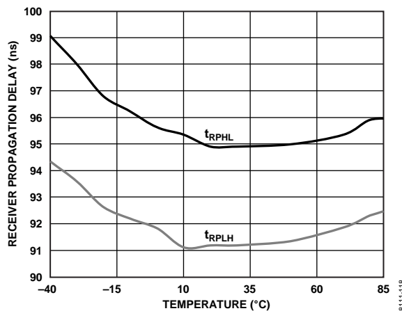
Figure 18. ADM2582E Receiver Propagation Delay vs. Temperature
