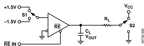
Figure 8. Receiver Enable/Disable
