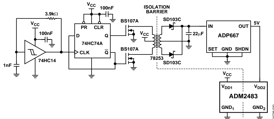
Figure 30. Isolated Power Supply Circuit
