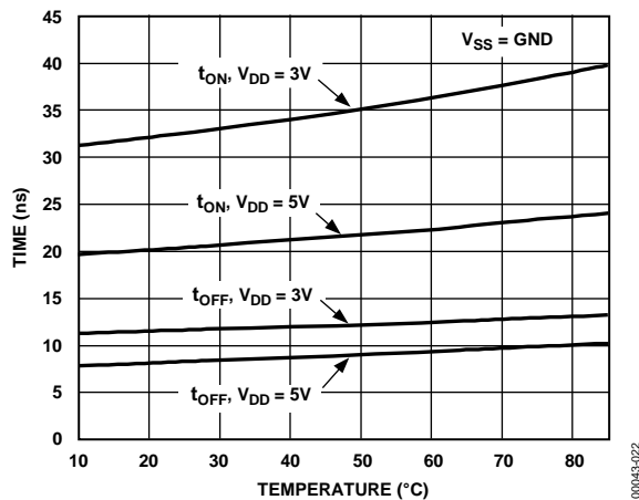
Figure 22. t_{ON}/t_{OFF} Times vs. Temperature for the ADG715
