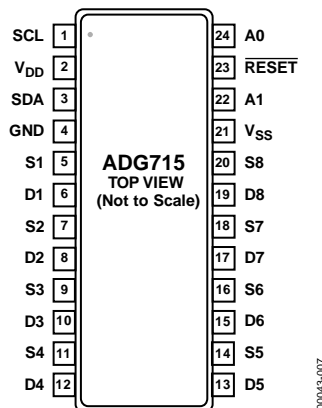
Figure 7. ADG715 Pin Configuration
