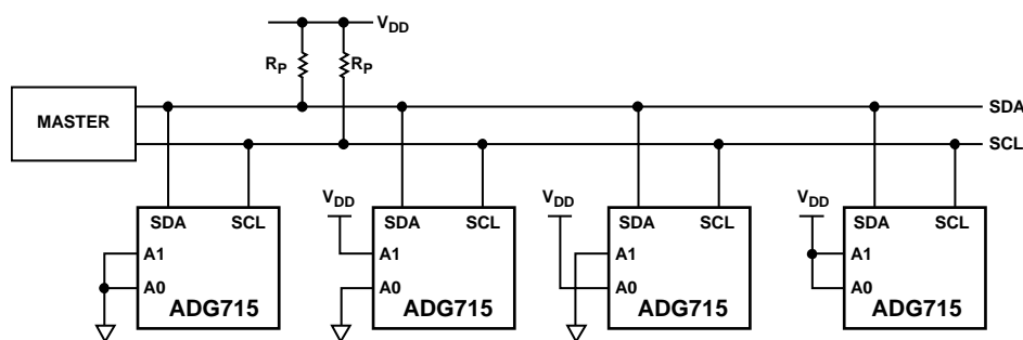
Figure 27. Multiple ADG715 Devices on One Bus
