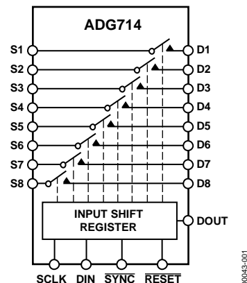
Figure 1. ADG714 Functional Block Diagram
