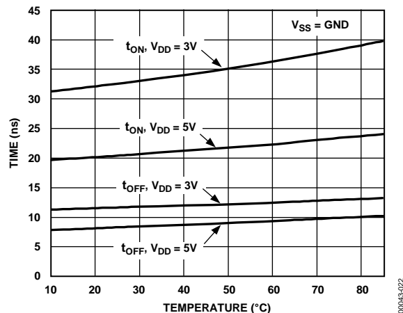
Figure 22. t_{ON}/t_{OFF} Times vs. Temperature for the ADG714
