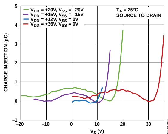
Figure 21. Charge Injection vs. Source Voltage, Source to Drain
