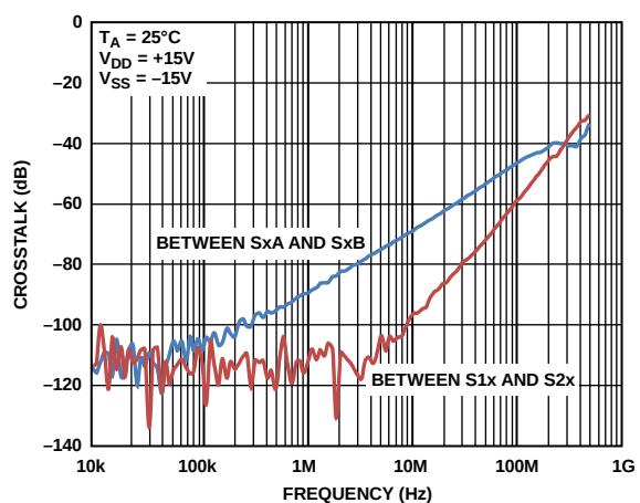
Figure 20. Crosstalk vs. Frequency, \pm 15 V Dual Supply
