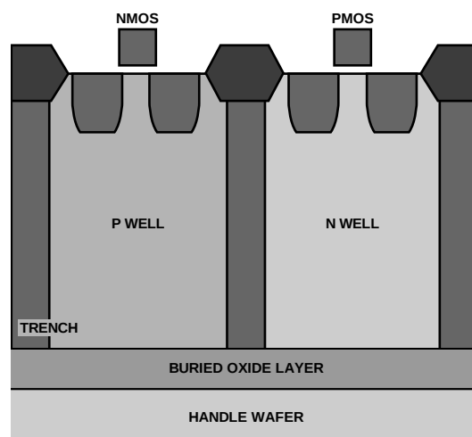
Figure 37. Trench Isolation
