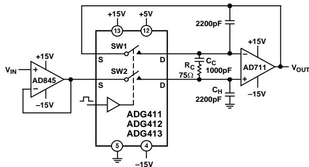
Figure 13. Fast, Accurate Sample-and-Hold
