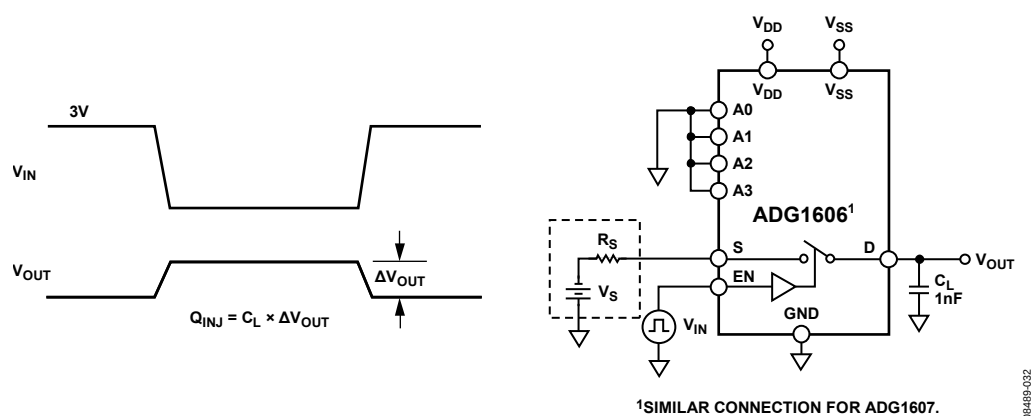
Figure 32. Charge Injection
