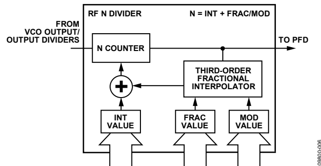
Figure 17. RF N Divider
