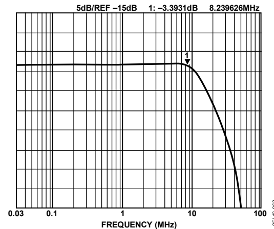
Figure 47. Video Reconstruction Filter Frequency Performance
