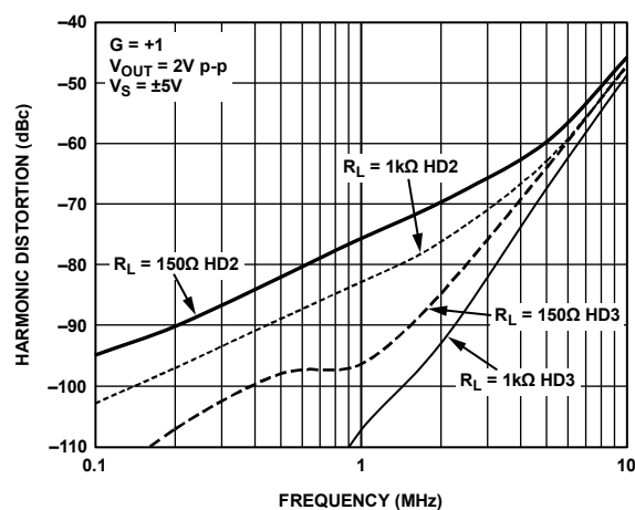
Figure 17. Harmonic Distortion vs. Frequency for Various Loads
