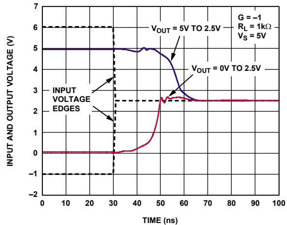
Figure 44. Overload Recovery
