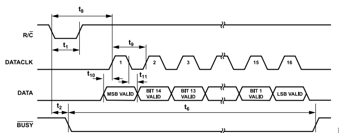
Figure 6. Serial Data Timing for Reading Previous Conversion Results with Internal Clock ( \overline{CS} , EXT/\overline{INT} and TAG Set to Logic Low)
