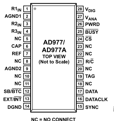
Figure 4. SSOP
