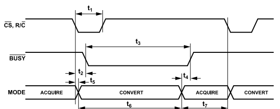
Figure 5. Basic Conversion Timing
