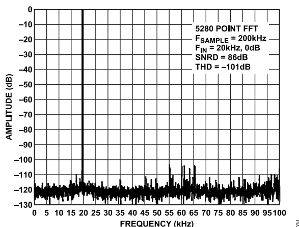
Figure 21. FFT Plot
