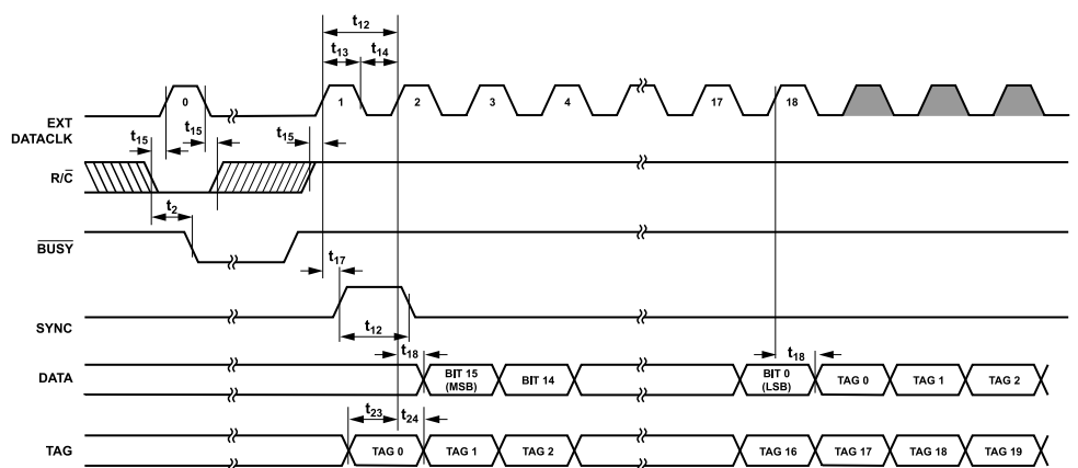
Figure 9. Conversion and Read Timing Using An External Discontinuous Data Clock (EXT/INT Set to Logic High, \overline{CS} Set to Logic Low)
