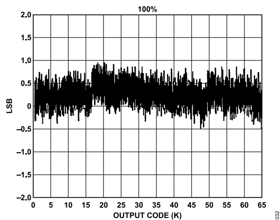
Figure 22. INL Plot
