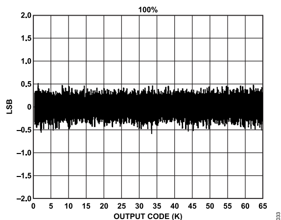
Figure 23. DNL Plot
