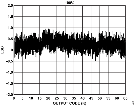
Figure 22. INL Plot
