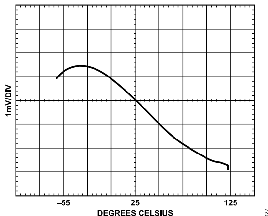
Figure 17. Reference Drift
