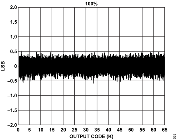
Figure 23. DNL Plot
