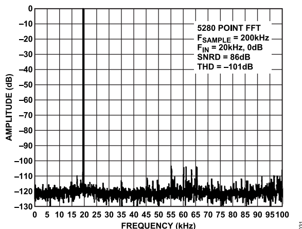
Figure 21. FFT Plot
