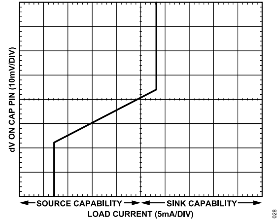
Figure 18. CAP Pin Load Regulation
