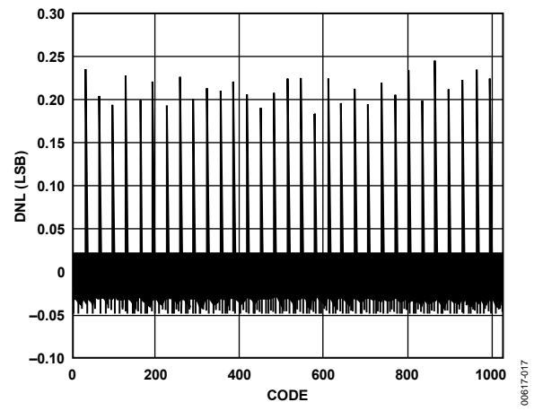
Figure 17. Typical DNL
