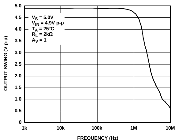
Figure 13. Closed-Loop Output Voltage Swing vs. Frequency
