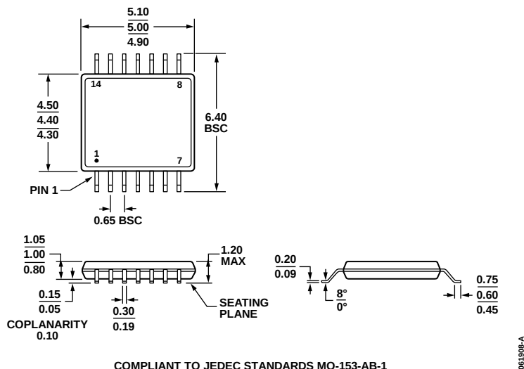
Figure 66. 14-Lead Thin Shrink Small Outline Package [TSSOP] (RU-14) Dimensions shown in millimeters and (inches)
