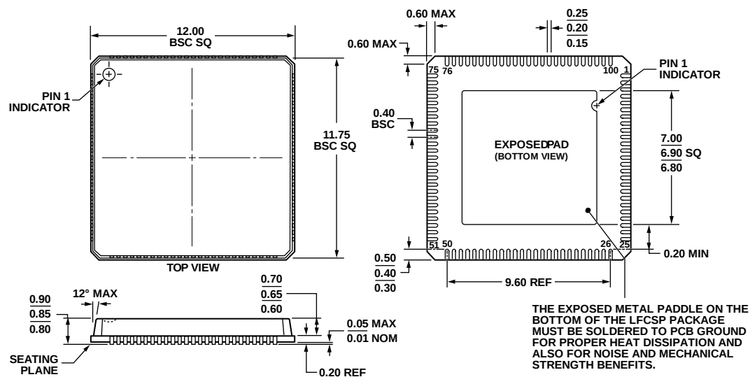
Figure 52. 100-Lead Lead Frame Chip Scale Package [LFCSP_VQ] 12 mm x 12 mm Body, Very Thin Quad (CP-100-1) Dimensions shown in millimeters
