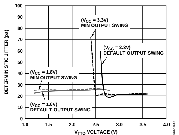
Figure 22. Deterministic Jitter vs. Output Termination Voltage (V TT0 )
