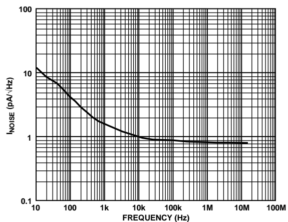
Figure 39. Current Noise vs. Frequency
