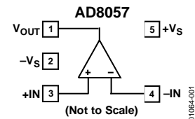
Figure 1. RT-5 (SOT-23)
