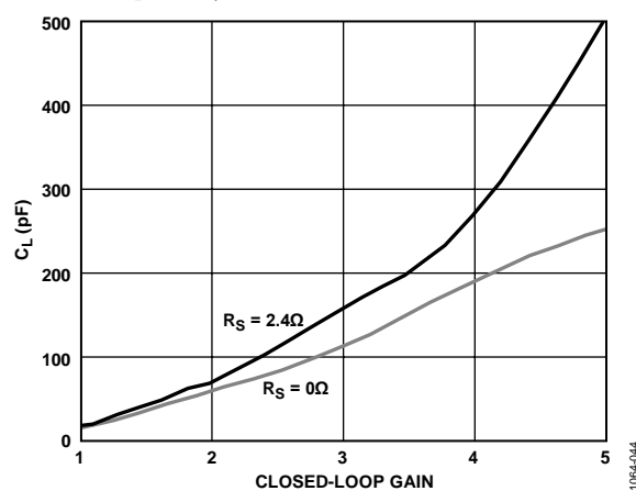
Figure 43. Capacitive Load Drive vs. Closed-Loop Gain
