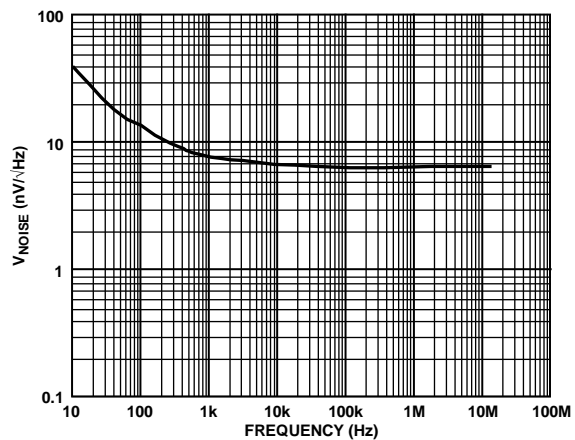
Figure 38. Voltage Noise vs. Frequency
