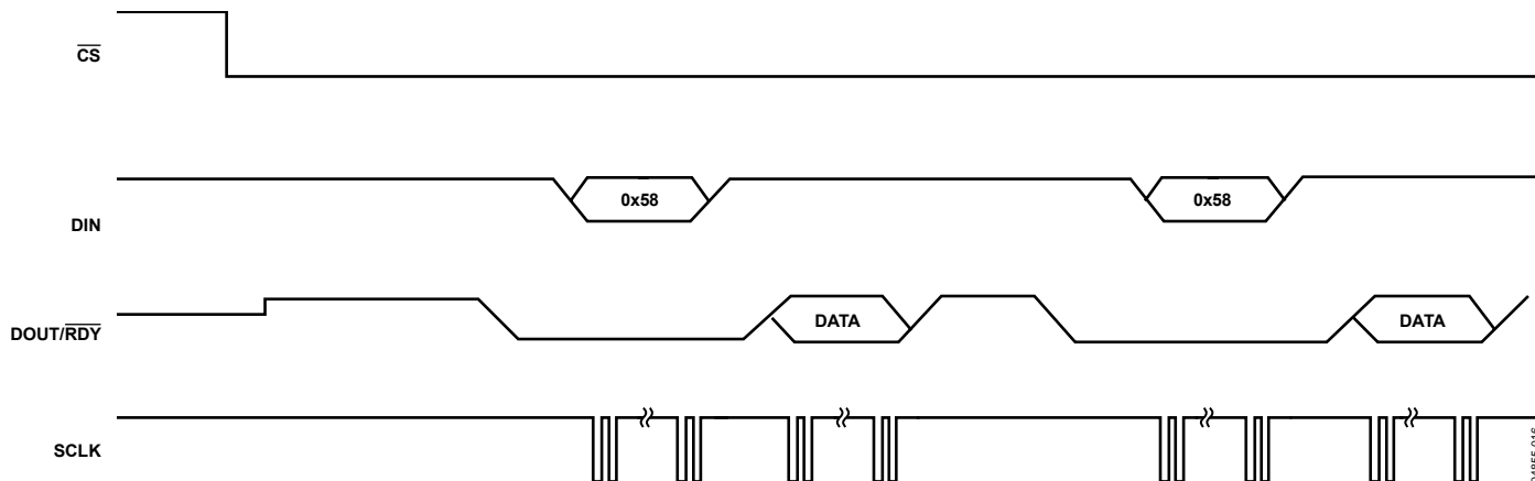
Figure 18. Continuous Conversion
