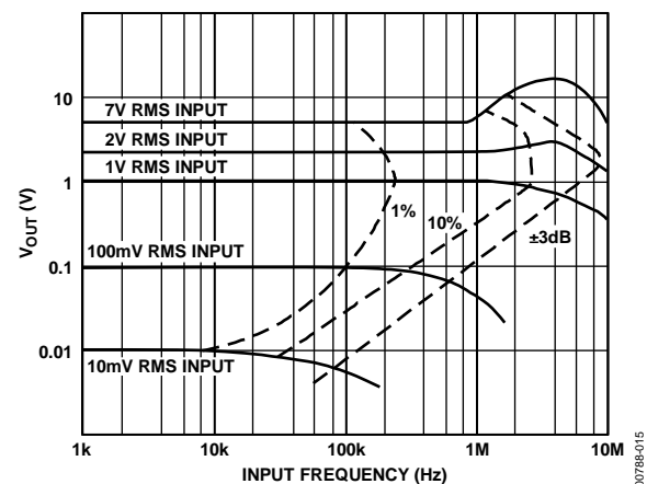
Figure 15. Frequency Response
