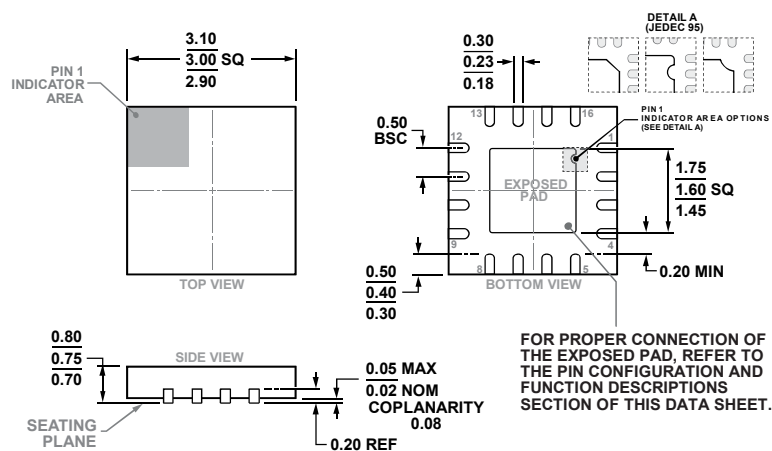
Figure 44. 16-Lead Lead Frame Chip Scale Package [LFCSP]
