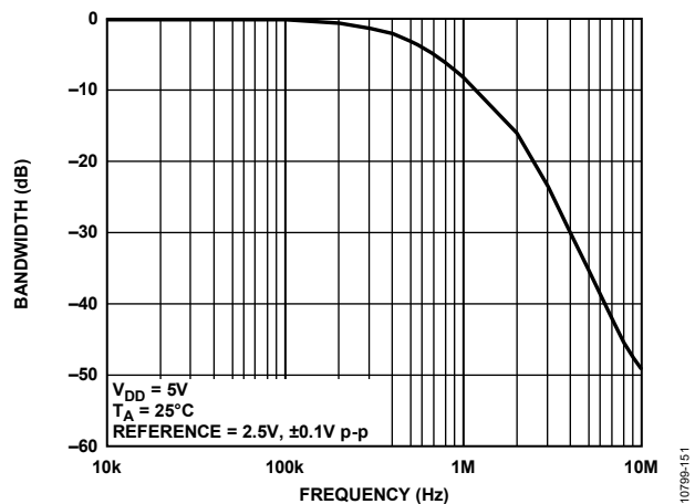
Figure 32. Multiplying Bandwidth
